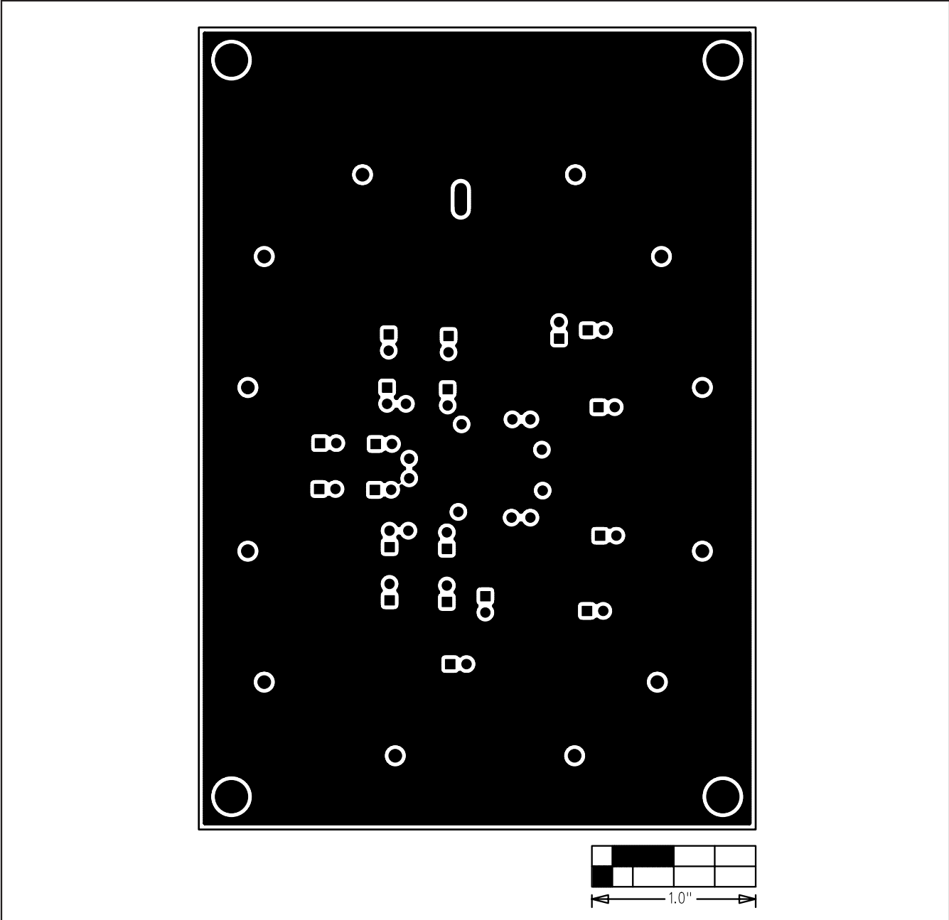
Figure 4. MAX11506 EV Kit PCB Layout—Solder Side
