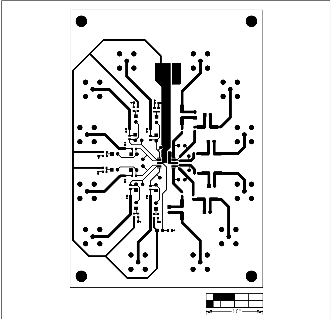
Figure 3. MAX11506 EV Kit PCB Layout—Component Side
