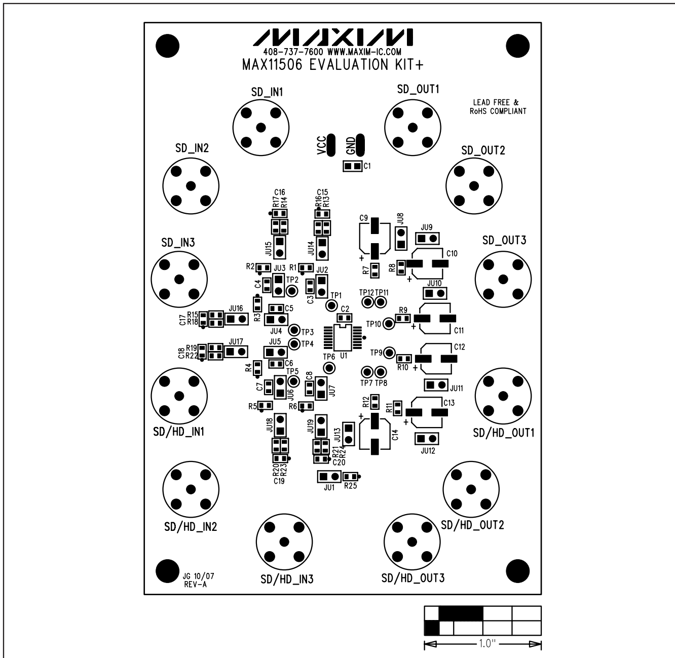
Figure 2. MAX11506 EV Kit Component Placement Guide—Top Silkscreen
